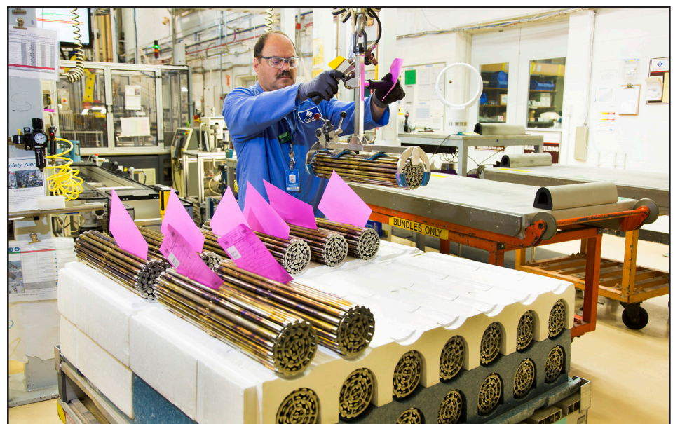
Packing fuel bundles for shipment at Cameco Fuel Manufacturing in Port Hope.
